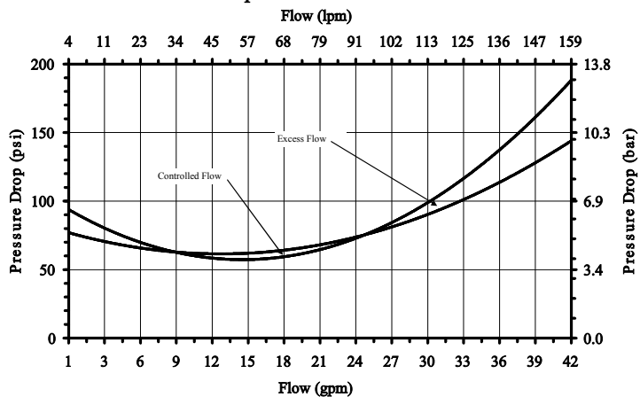
Pressure Drop vs. Flow for FC Series
