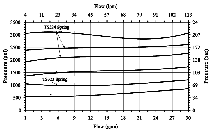
Pressure vs. Flow for FCB51
